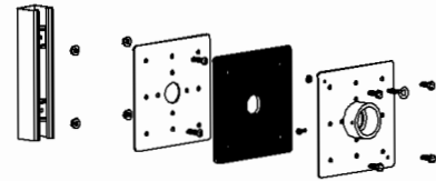
Exploded view of the NB-UIM-96-US attached to Unistrut
