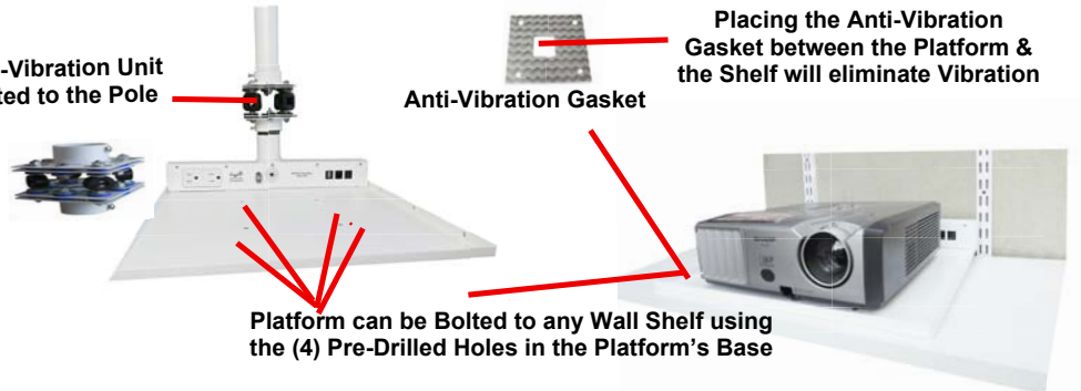
Projector Platform with Unistrut
