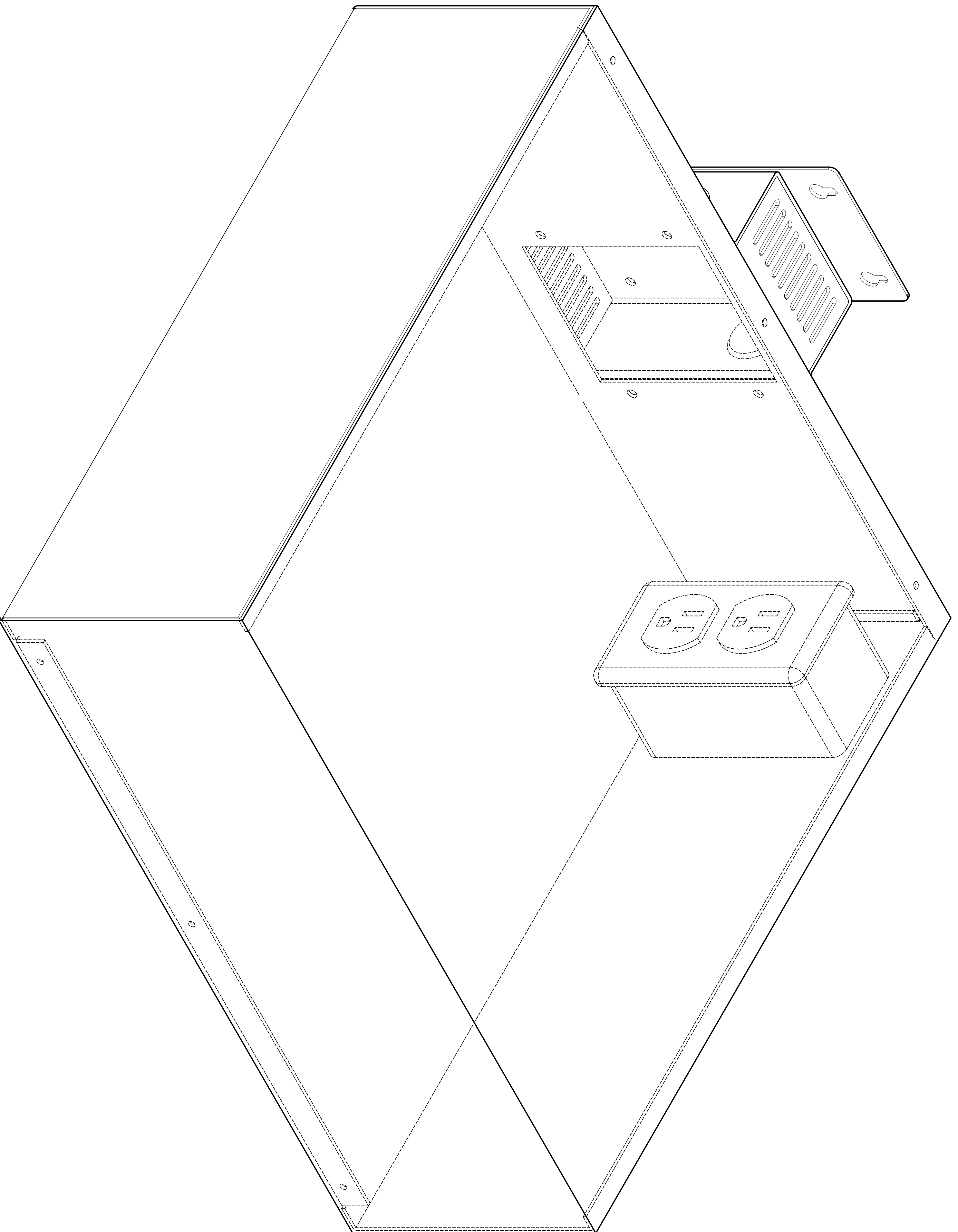
ISOMETRIC VIEW
