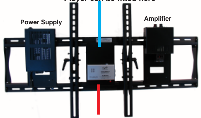
A typical Outboard Installation of our Amplifier & Power Supply with the addition of a Limpet and space for a Signage Player and /or other Device
