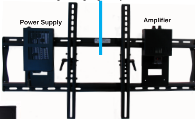
Peerless Smartmount® Model ST 650 showing a typical Outboard Installation
